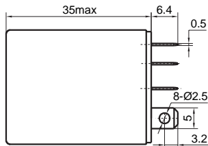
Outline Dimensions
